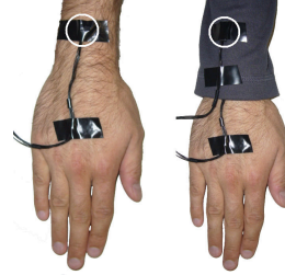
Figure 4: Setup to calculate the relative orientation error for a garment-attached acceleration sensor (right) relatively to a reference sensor (left) during the execution of postures. The position of both sensors is marked with white circles.
