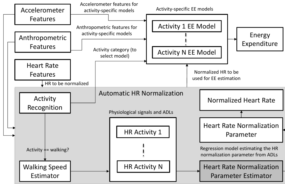
Figure 1. Overview on the activity-specific EE estimation and extension for automatic HR normalization using an HR normalization parameter estimated from ADLs. Accelerometer features are used for activity recognition, walking speed estimation and EE models. HR in specific activities (1..N, e.g. lying and walking at a certain speed) is used to estimate the HR normalization parameter. The HR normalization parameter is then used to normalize HR and predict EE with higher accuracy.
