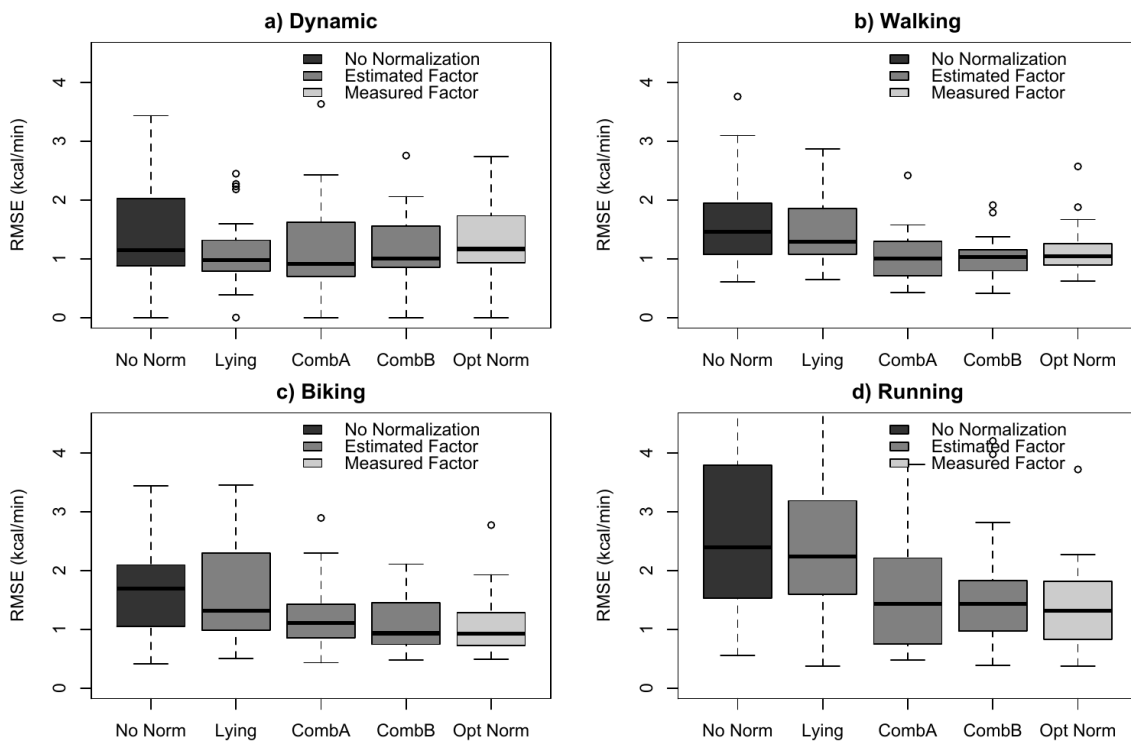
Figure 4. Algorithm performance in terms of RMSE of EE estimations during different moderate to vigorous activity clusters ( a to d show dynamic activities, e.g. household, and walking, biking and running activities) where HR is not normalized (No Norm), normalized using lying data only, and normalized using ADLs included in CombA and CombB . Normalization performed using the measured HR normalization parameter (Opt Norm) is also shown for comparison. The first column of each subplot shows performance of state of the art activity-specific EE models combining accelerometer and heart rate features, but without HR normalization.
